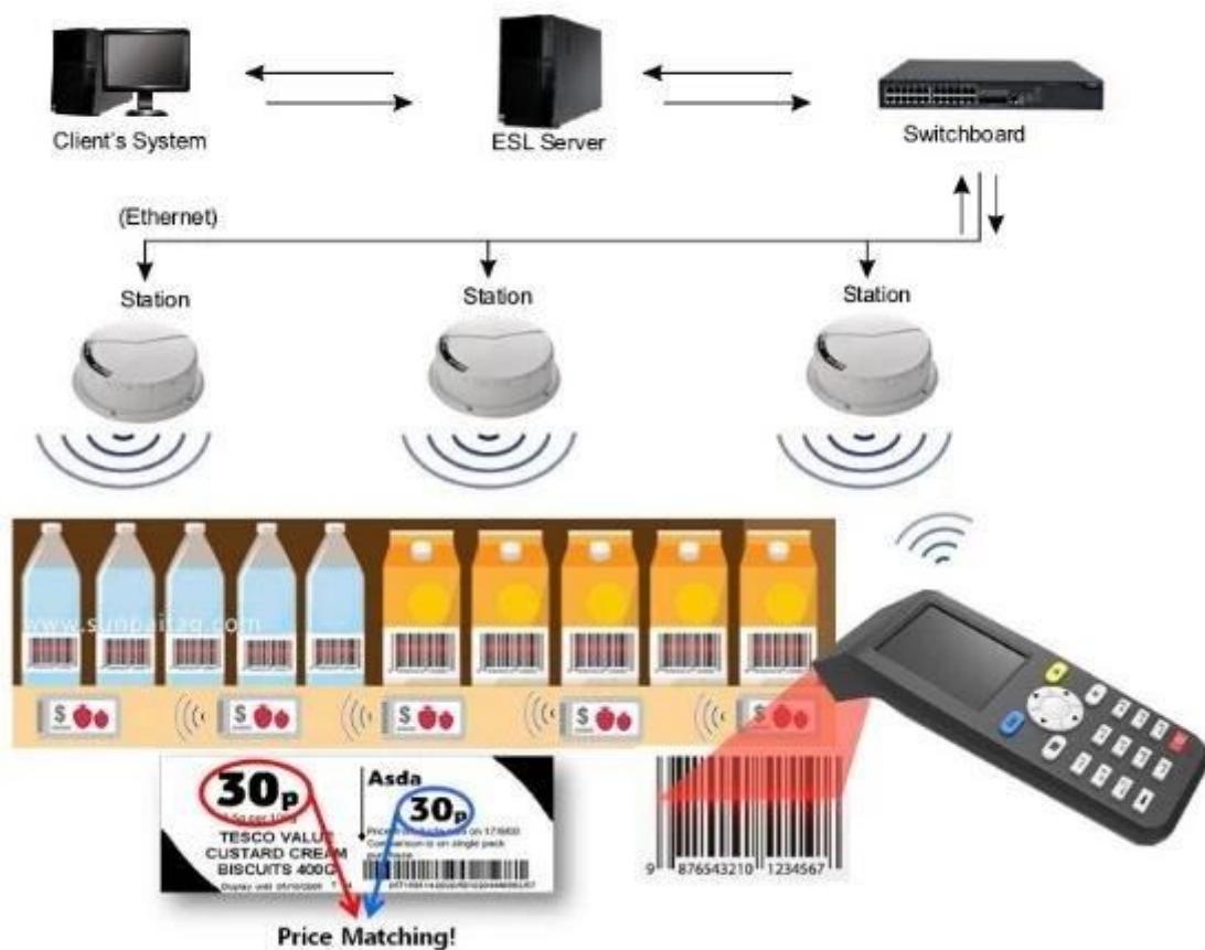
Electronic Shelf Label System (ESLs) Schematic Diagram
